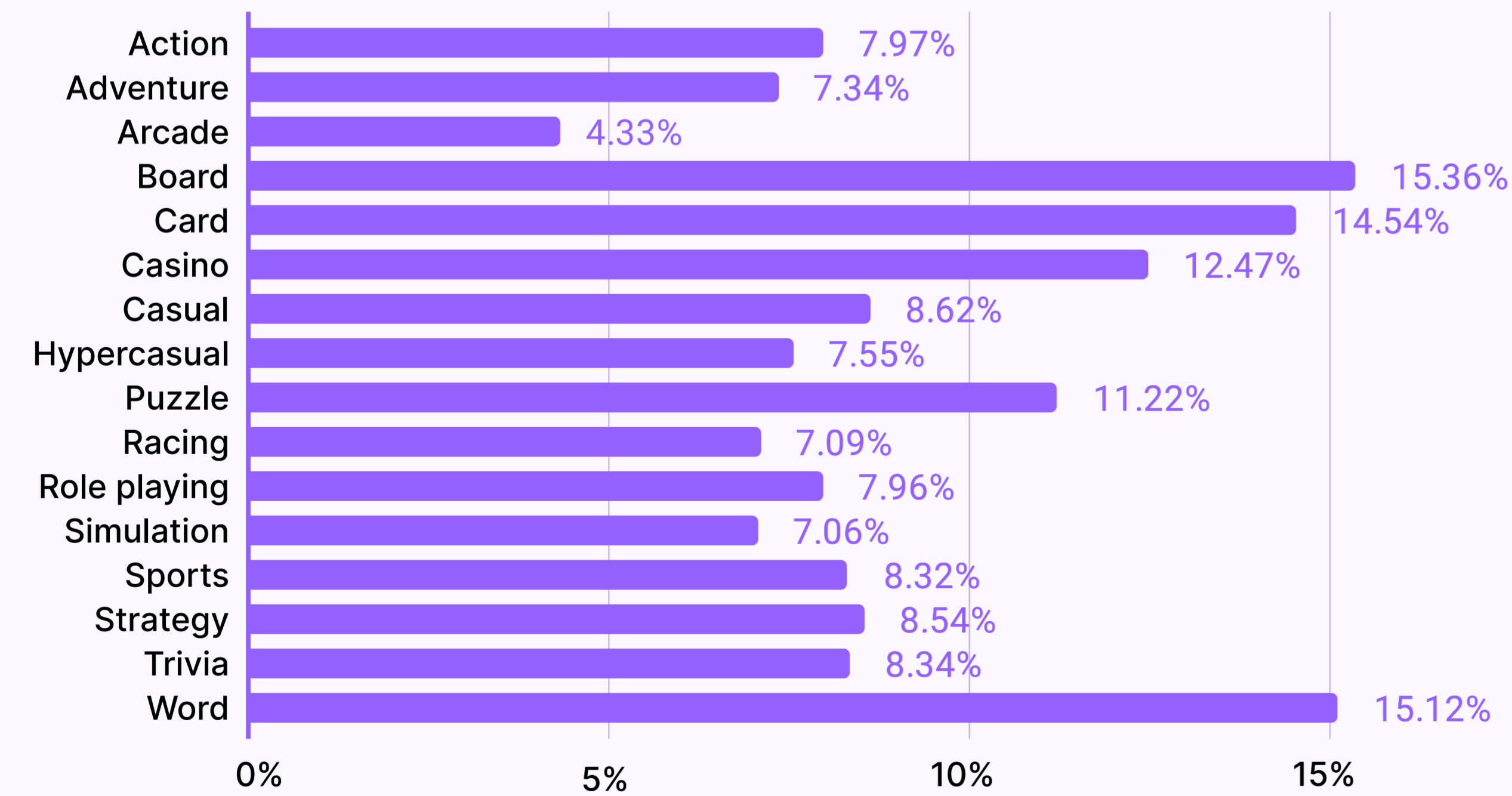
CHART 5.5: D7 retention has more separation.
