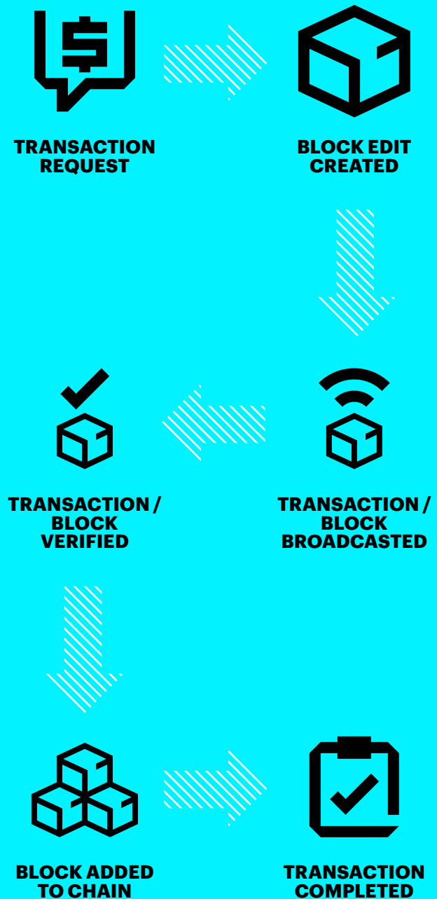
Figure 7—Blockchain Diagram.
