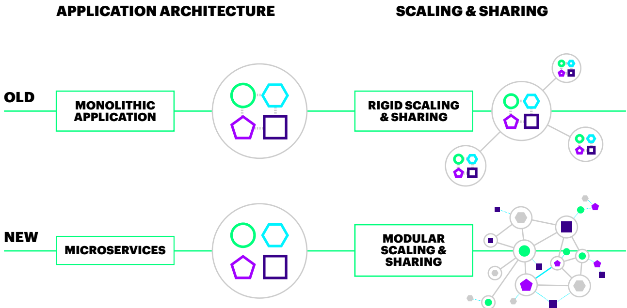
Figure 6—Microservices Diagram.
